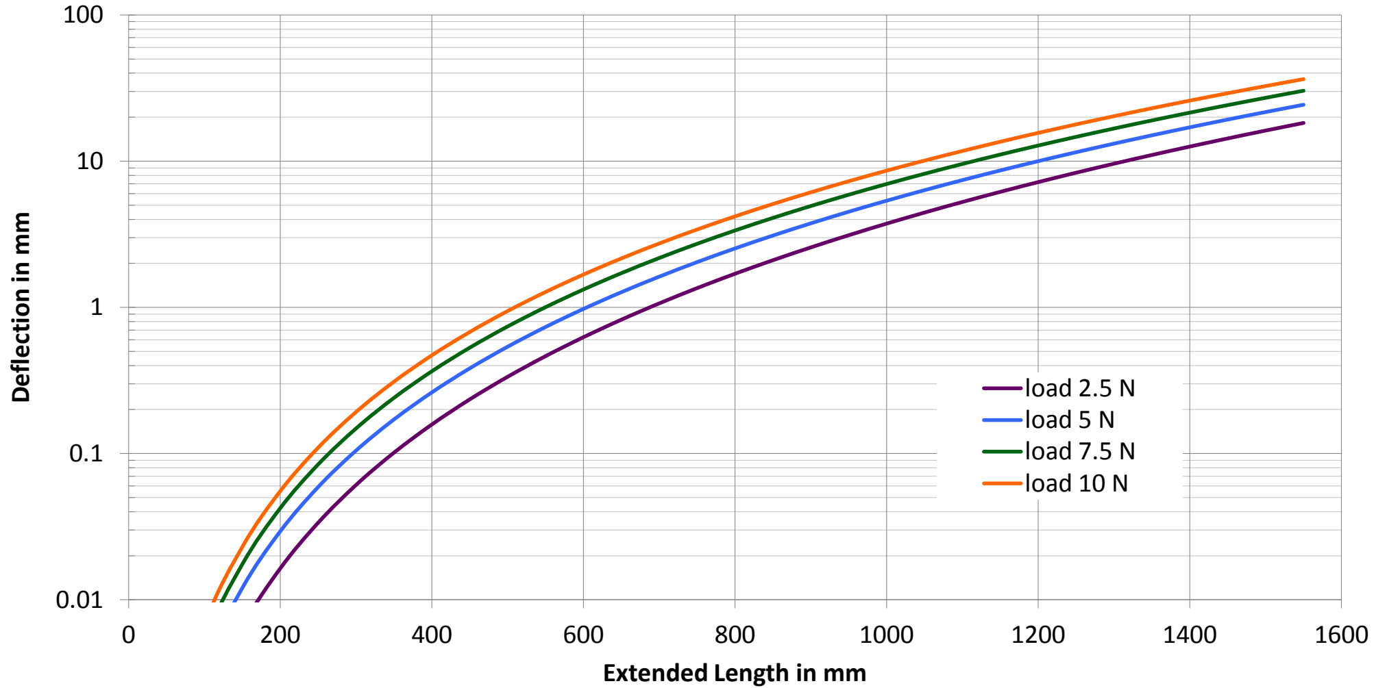
RMD / RMDG Deflection vs Extended Length at different Loads
