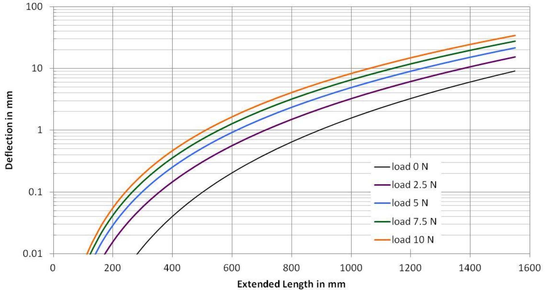
RMDS Deflection vs Extended Length at different Loads
