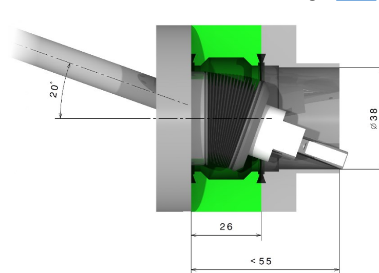
Bellows Protection Flange: BP40
